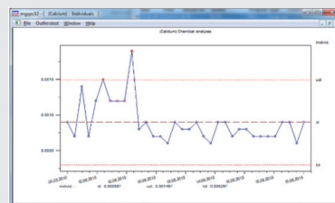
SPC software
